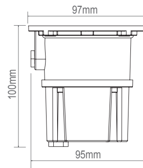
LED body
